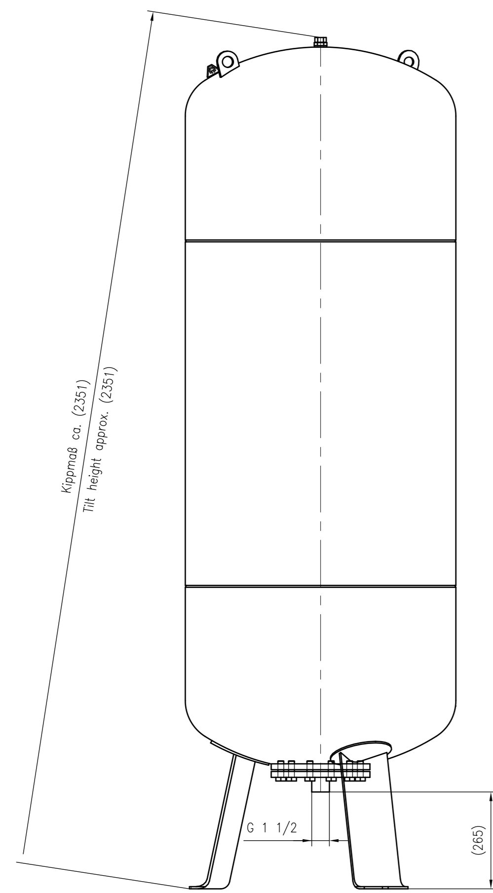
Side view
