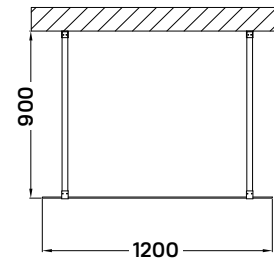
ASTRO 120 WALK-IN ZUHANYFAL
