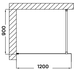
ASTRO 120 CORNER WALK-IN ZUHANYFAL
