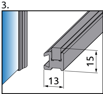
Balos kabin Variant L
