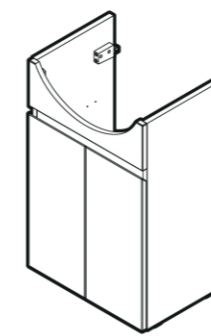
H453101038xxx1 446x315x696
