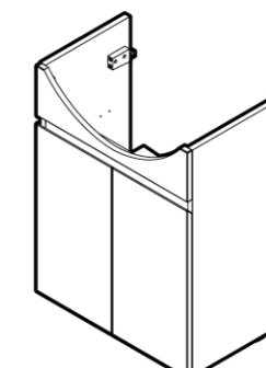
H453121038xxx1 540x315x696
