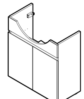
H453141038xxx1 670x315x696
