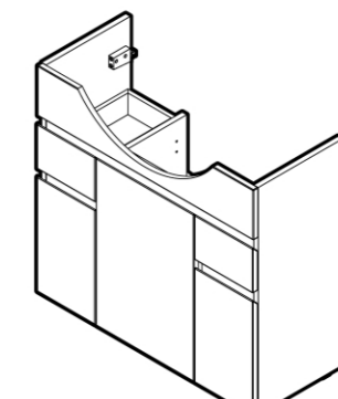
H453152038xxx1 770x315x696
