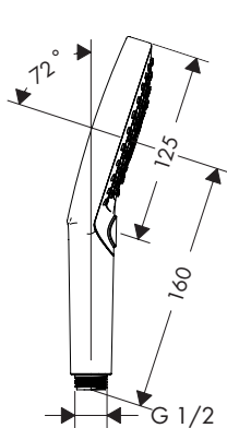
Raindance Select S 120
