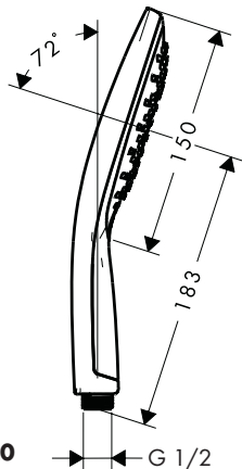
Raindance Select S 150
