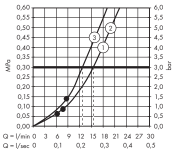
Raindance Select S 120 26530000 / 26530400
